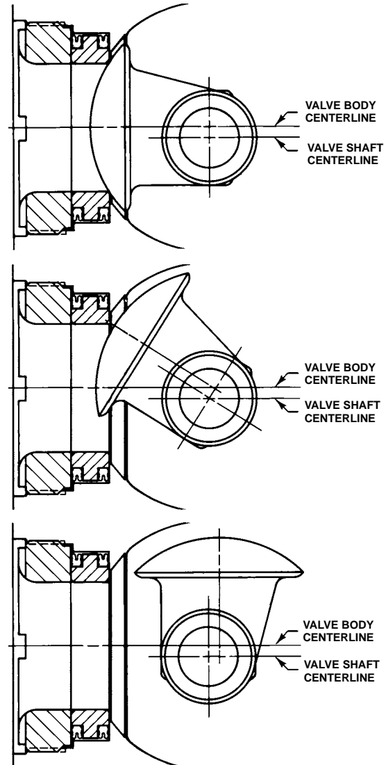
Figure 5. Eccentric Rotation
