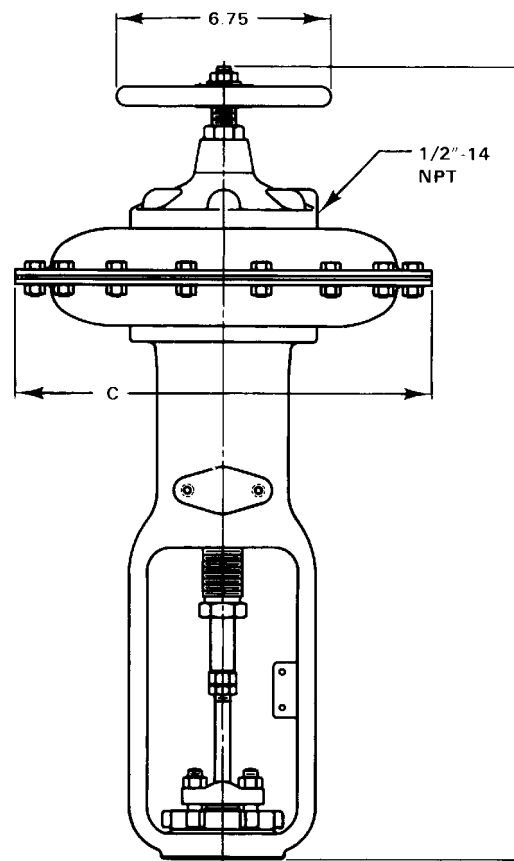
Figure 2. Actuator Dimensions, Inches (also see table 5)
