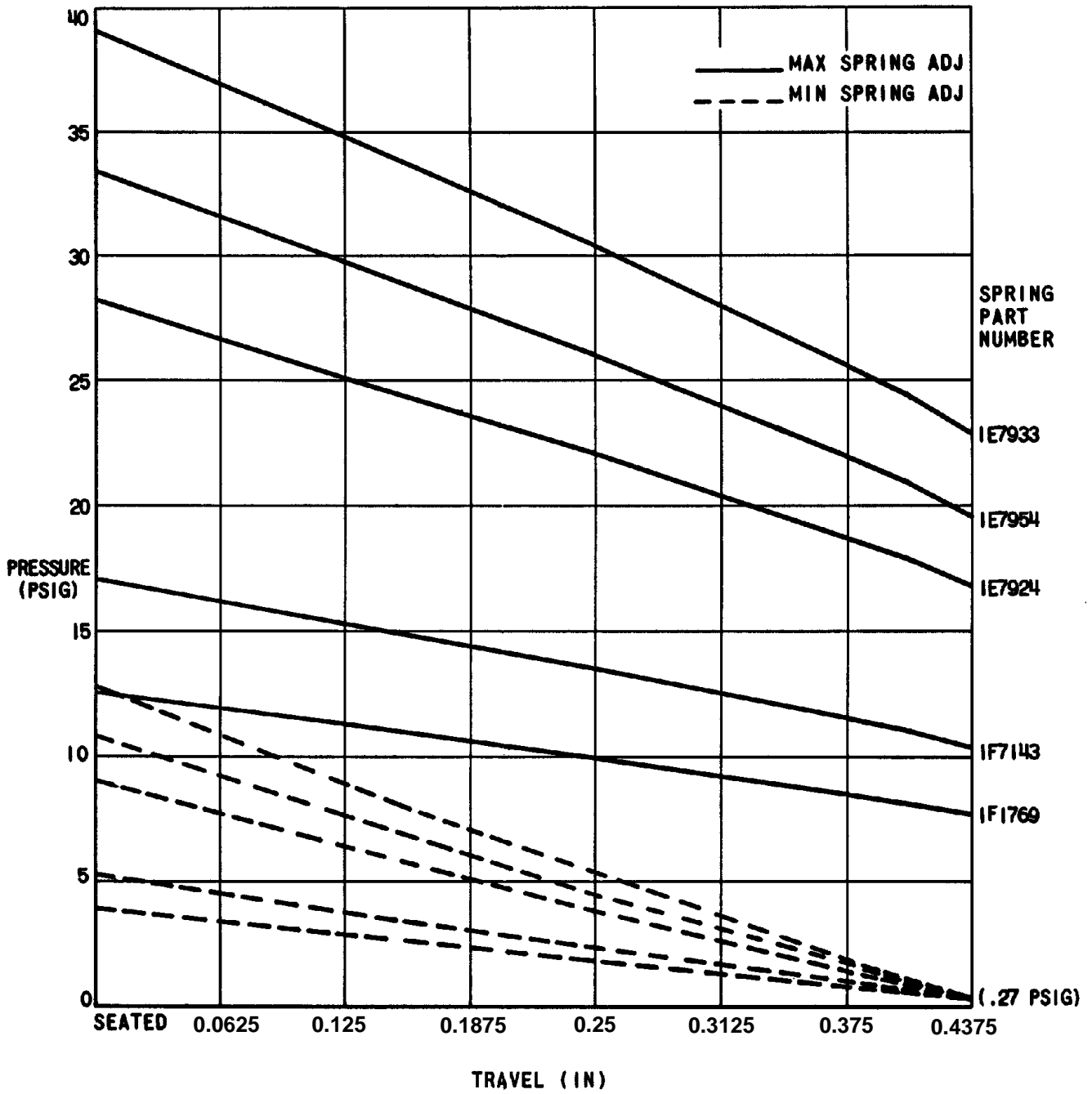
Figure 10. 655 ED, #40 Casing, Diaphragm Pressure versus Valve Travel
