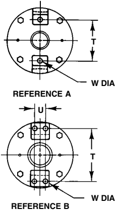
ACTUATOR/VALVE BODY MOUNTING DIMENSIONS
