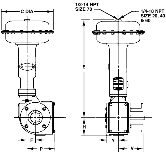
TYPE 1052 SIZE 20, 40, 60, AND 70 ACTUATOR
