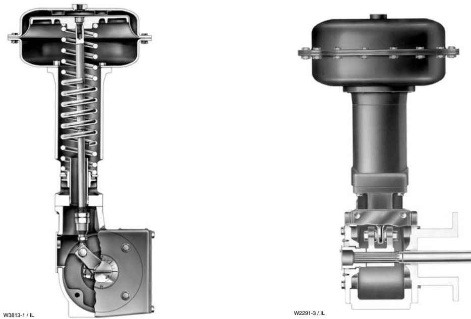
Figure 3. Sectional Views Typical of Size 40, 60, and 70 Actuators
